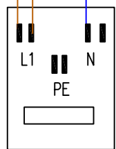
TERMINAL BOX
