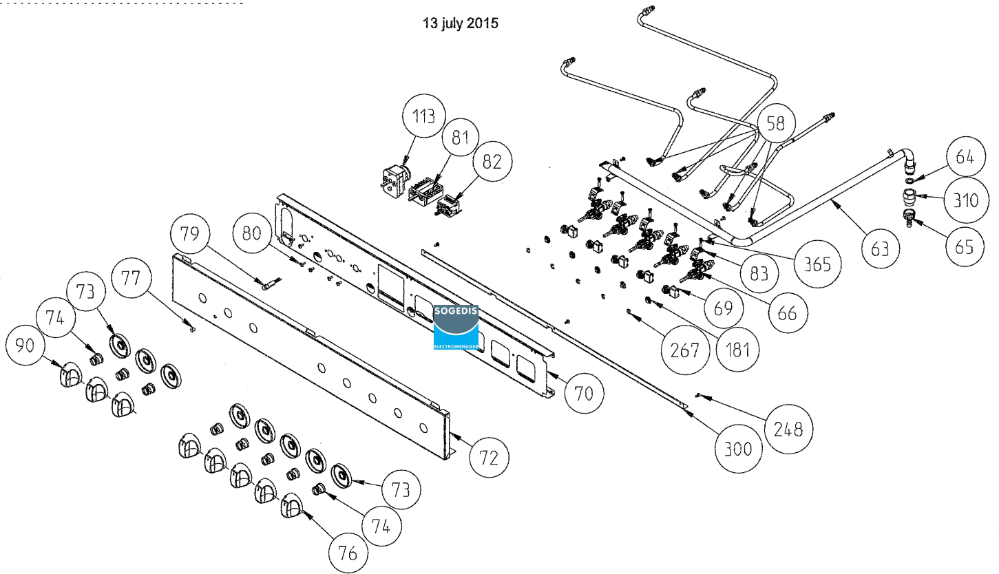
5 GAS OVEN ELECTRIC MECHANIC TIMER CONTROL PANEL ASSEMBLY
