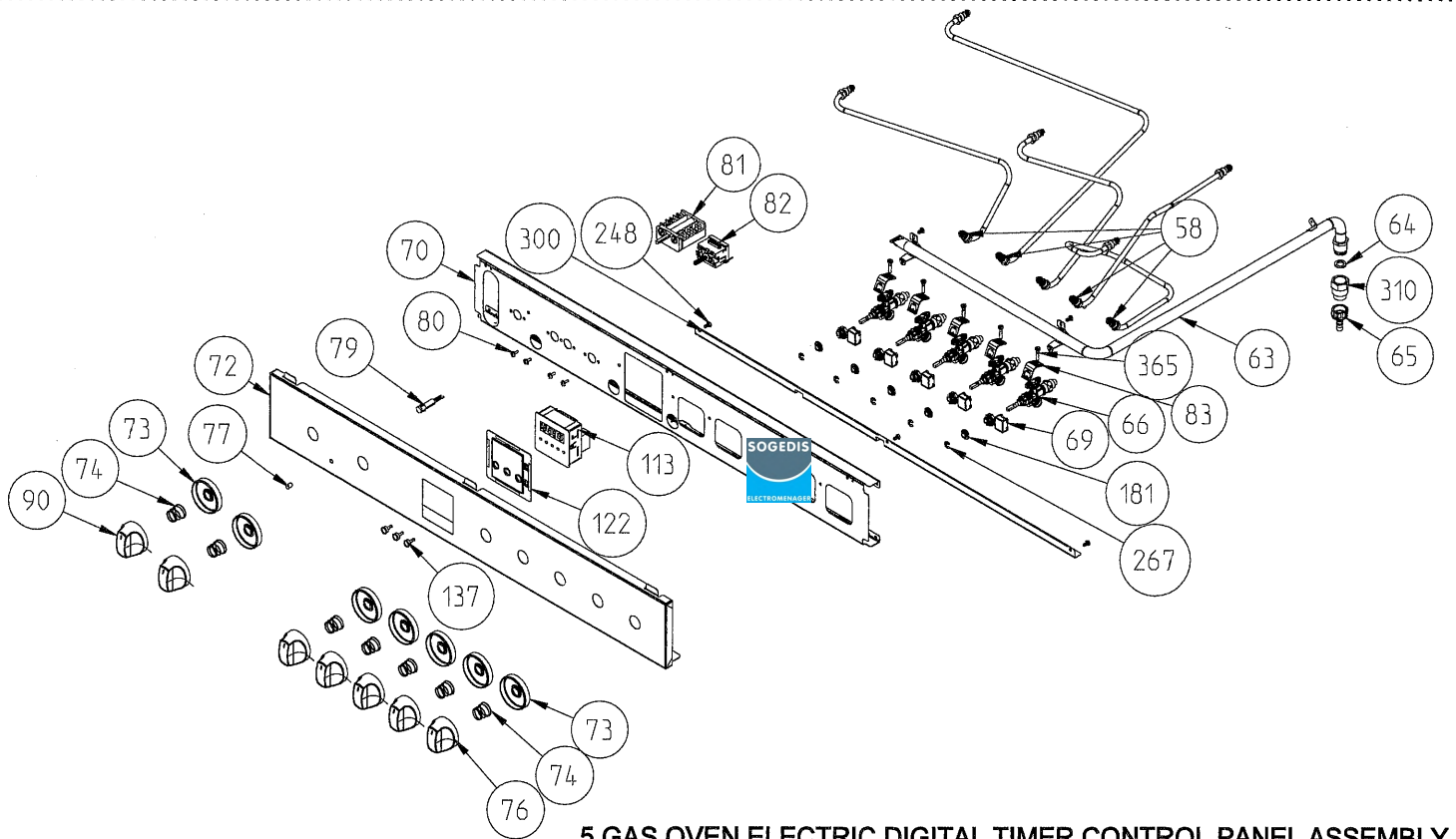
5 GAS OVEN ELECTRIC DIGITAL TIMER CONTROL PANEL ASSEMBLY
