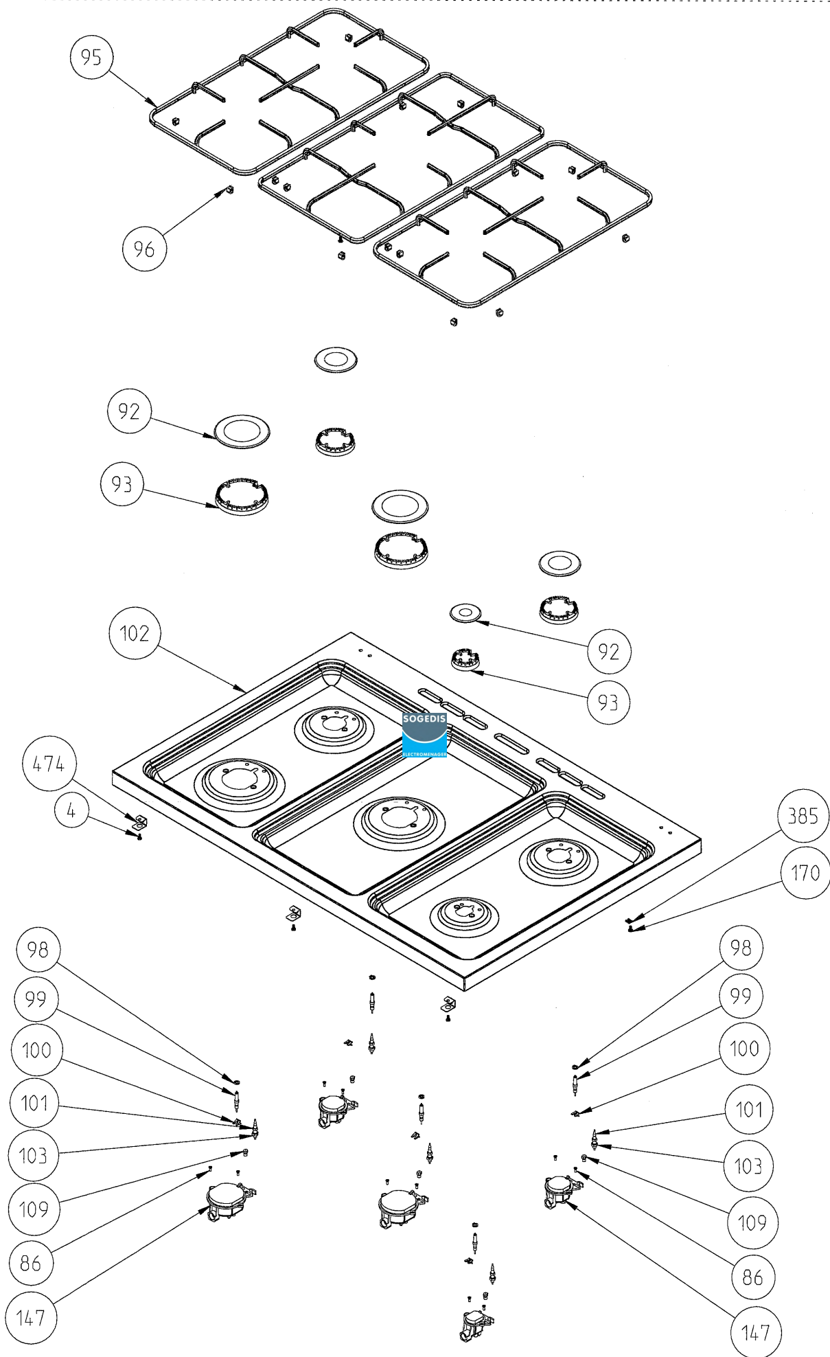
5 GAS COOKTOP ASSEMBLY
