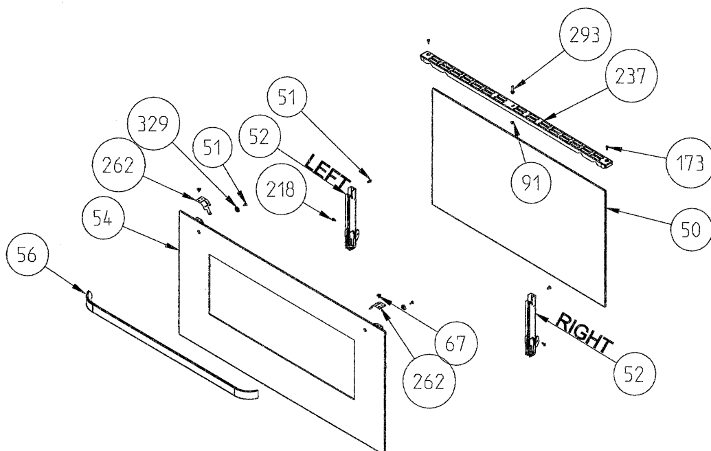
POSITION NUMBER 377 PROFILE OVEN DOOR WITH 2 GLASSES BIG INNER GLASS
